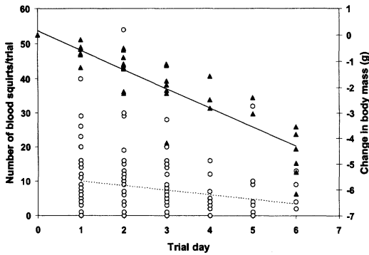
Fig. 3. Regression of number of lizard ( Phrynosoma cornutum ) blood squirts per trial (open circles, dashed line; r^2 = 0.20 , P < 0.05 ) and loss of mass (g) (solid triangles, solid line; r^2 = 0.81 , P < 0.001 ) on trial day.
