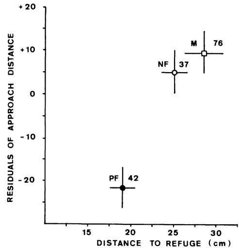
Fig. 4. Plot of the distance to refuge versus residuals of approach distance (from the regression on refuge distance), for males (M), pregnant females (PF), and nonpregnant females (NF). Mean values ( \pm one standard error) and sample sizes are shown.
